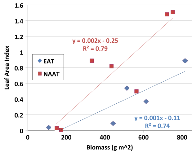
Figure 9. Leaf area index versus total aboveground biomass along the North America Arctic transect (NAAT) and the Eurasia Arctic Transect (EAT).
